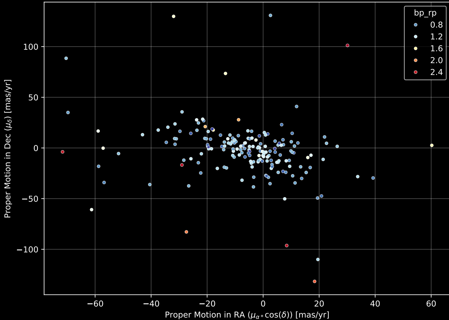
APOGEE DR17 Field: [063+47_MGA] Proper Motion Diagram (n= 183)
