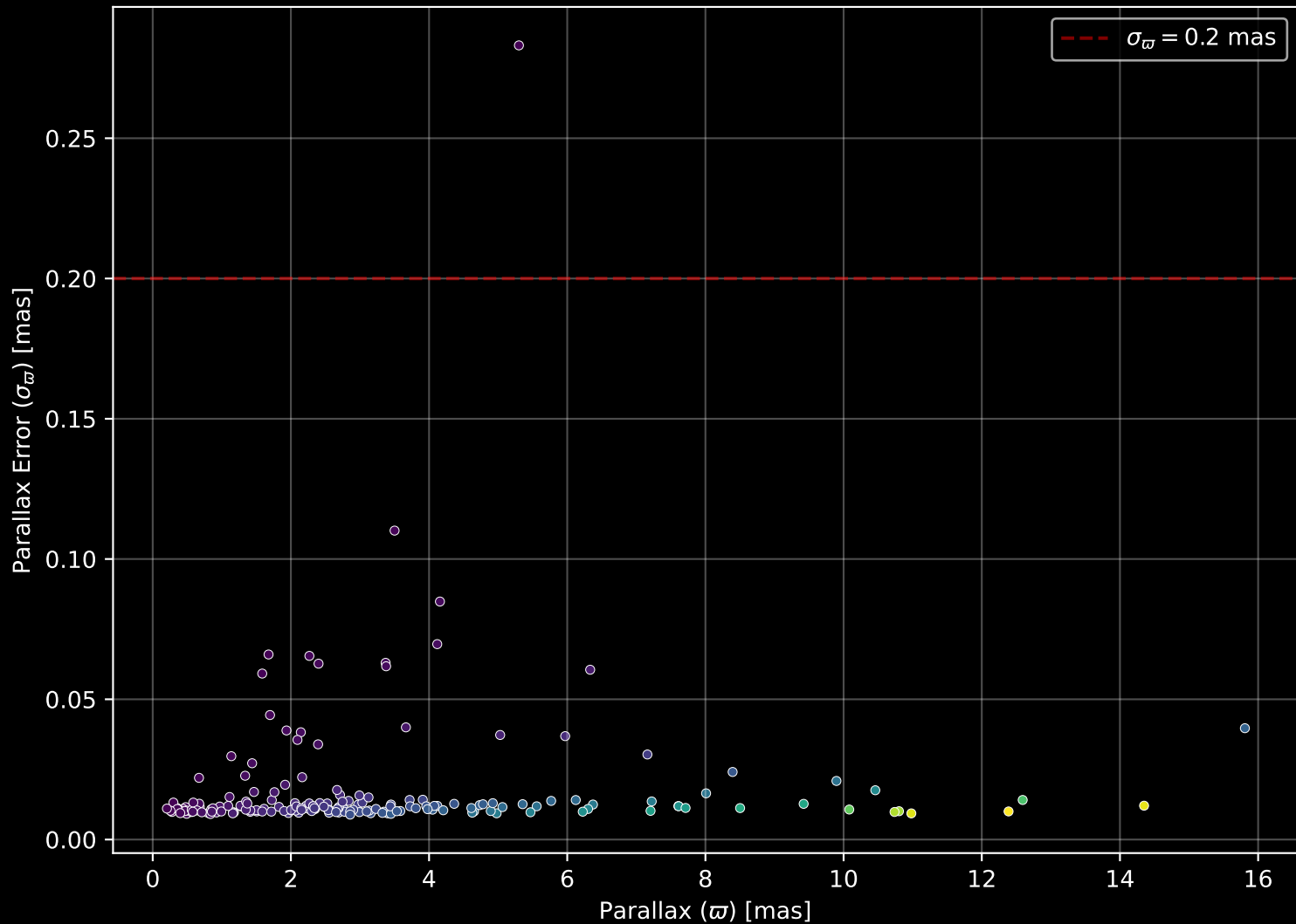
APOGEE DR17 Field: [063+47_MGA] Parallax Quality (n= 183)
