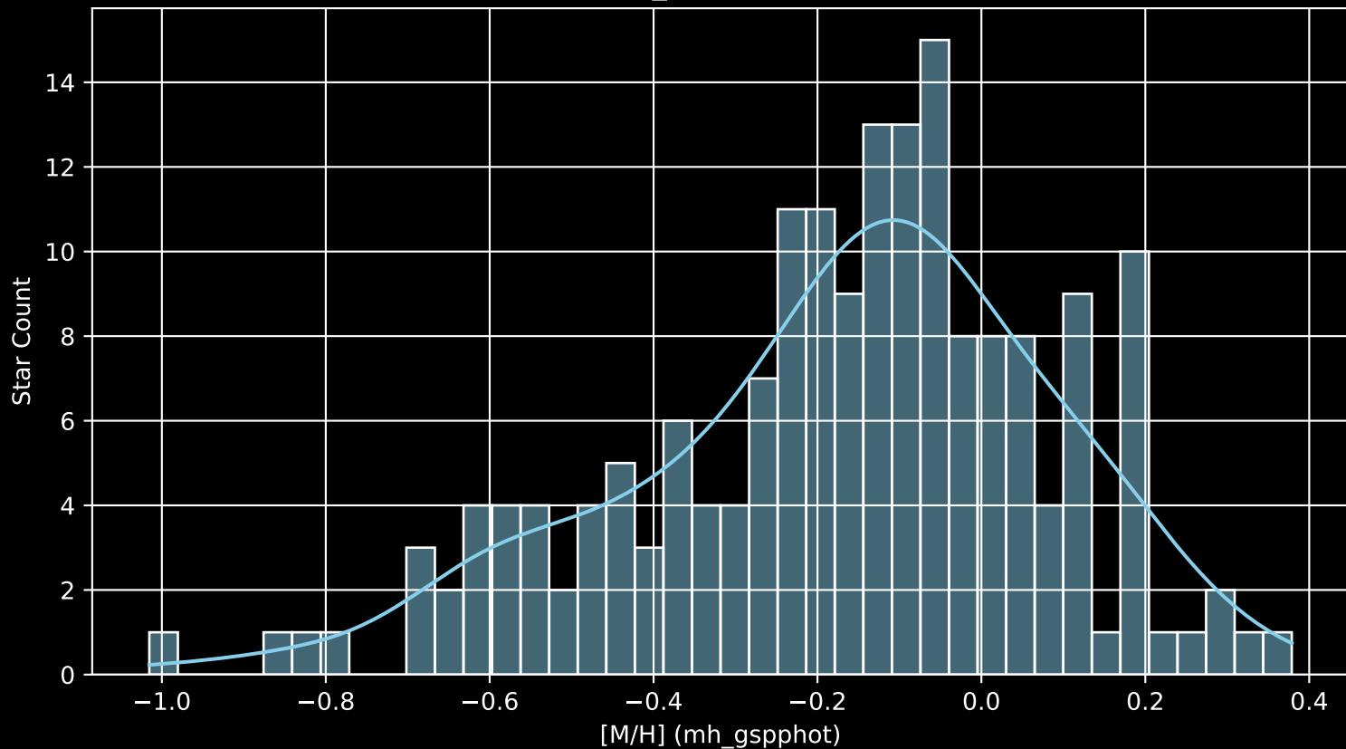
APOGEE DR17 Field: [063+47_MGA [M/H] (mh_gspphot) (n= 182)
