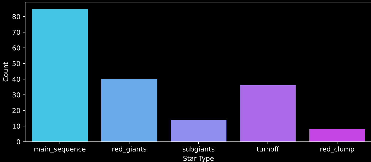
APOGEE DR17 Field: [063+47_MGA] Count plot of Star Type
