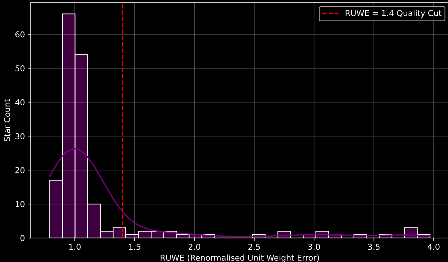
GAPOGEE DR17 Field [063+47_MGA] RUWE Distribution (n= 175)
